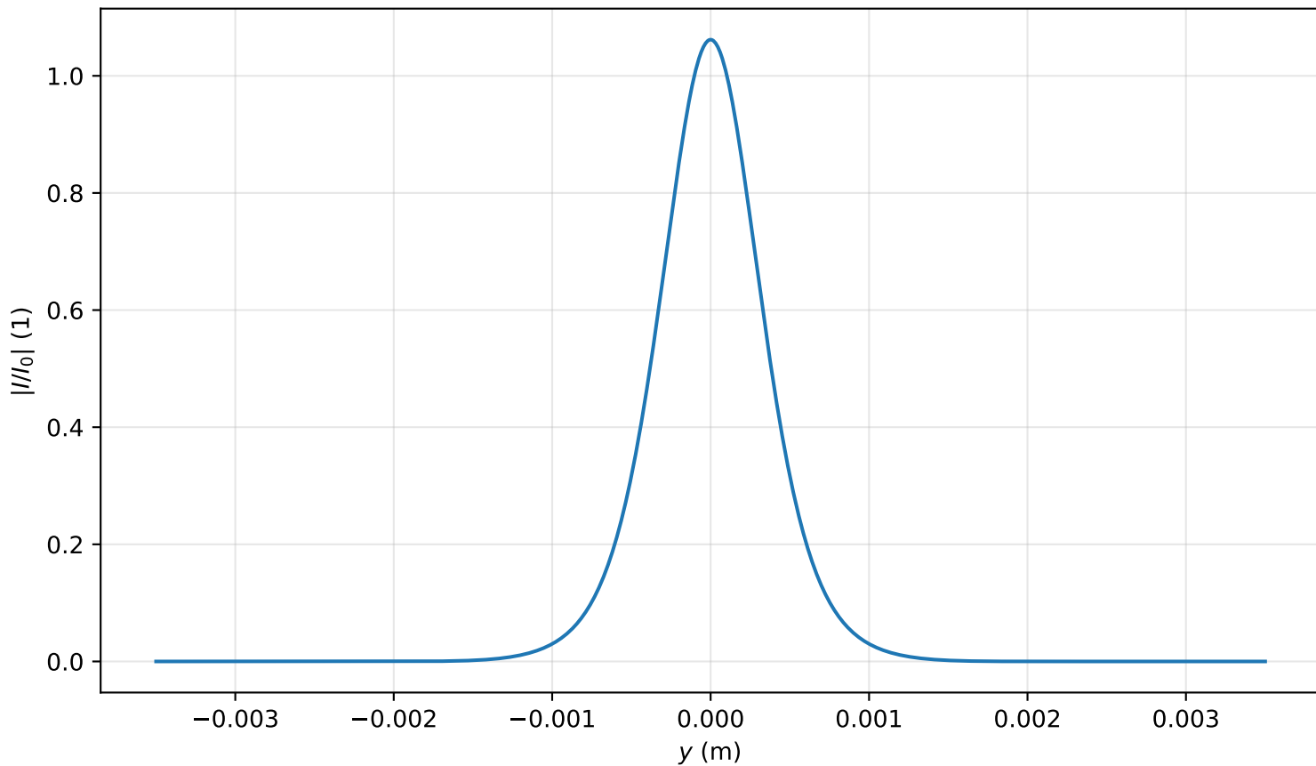
Intensity profile I(x=0, y, z=1.513)/I_0 , P_{in}=0.6P_{cr} , artificial time
